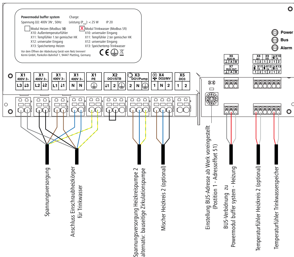
Abb. 13: Klemmenplan Powermodul buffer system - TWE
