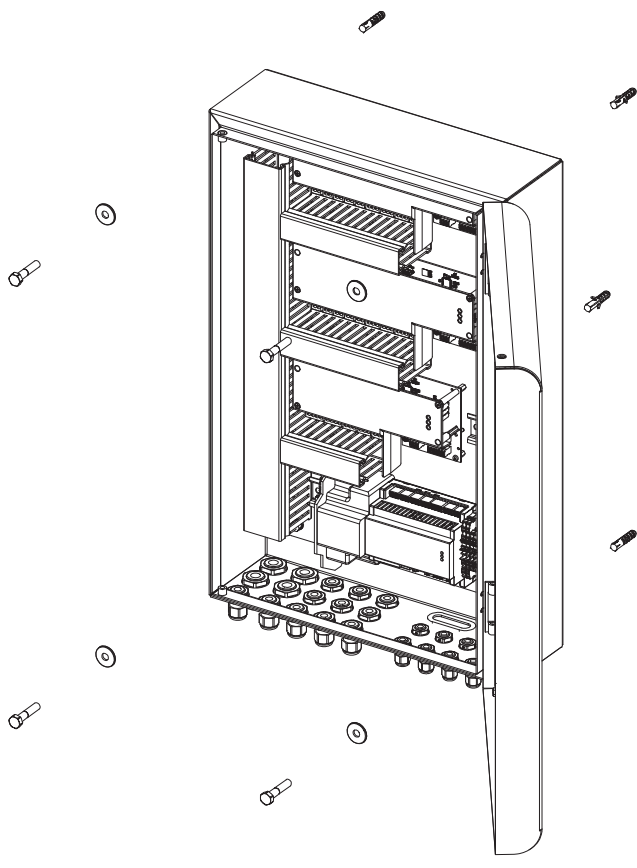
Abb. 5: Wandmontage
