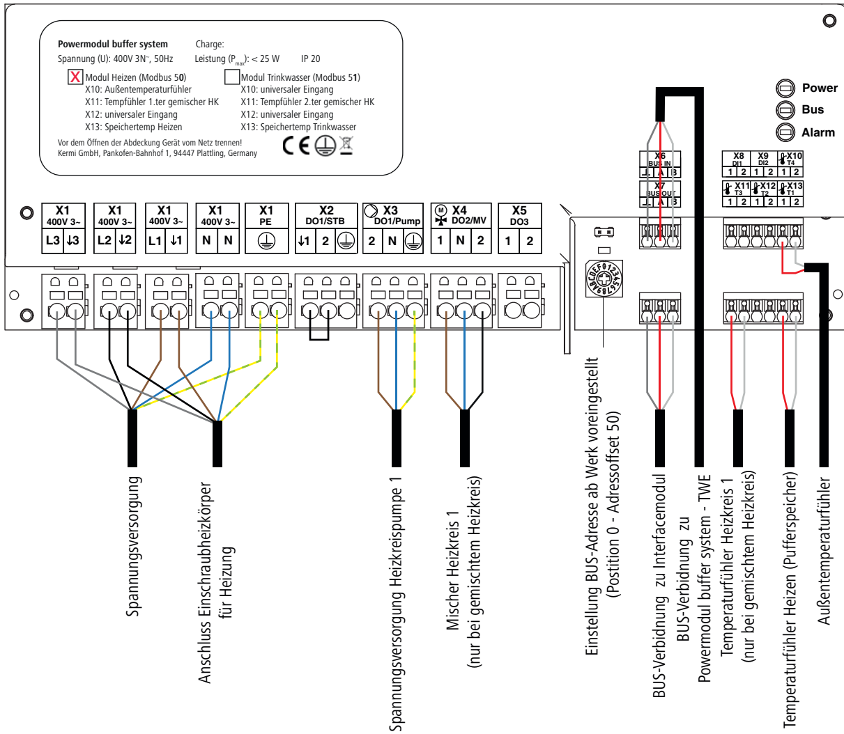
Abb. 12: Klemmenplan Powermodul buffer system - Heizung
