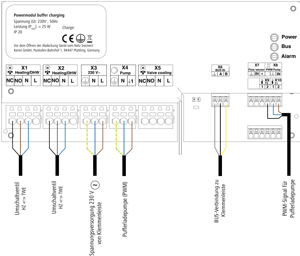
Abb. 11: Klemmenplan Powermodul buffer charging
